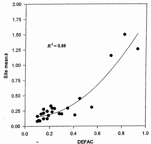
Fig. 1 The best predictor of the site mean k -value was a quadratic relationship using DEFAC from the CENTURY model.
