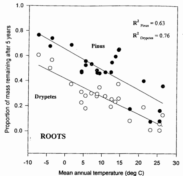
Fig. 3 Relationship between the proportion of mass remaining after 5y and MAT for fine roots decomposing at the LIDET sites. Lines are linear least-squares fits. The two saltmarsh sites have been excluded in this analysis. Both regressions are significant at P=0.0001 .
